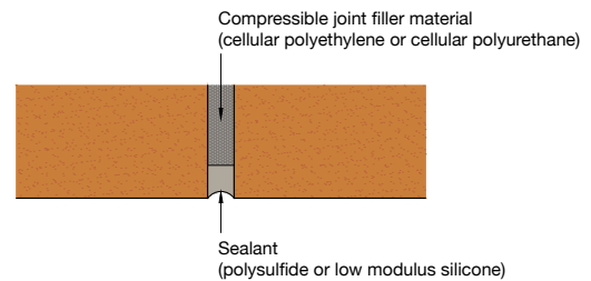
Typical Movement Joint Detail Plan
