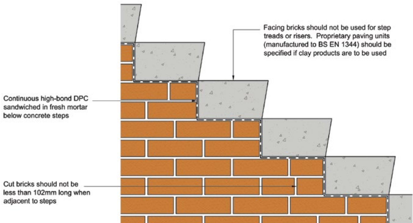
Step Flank Walls Elevation
